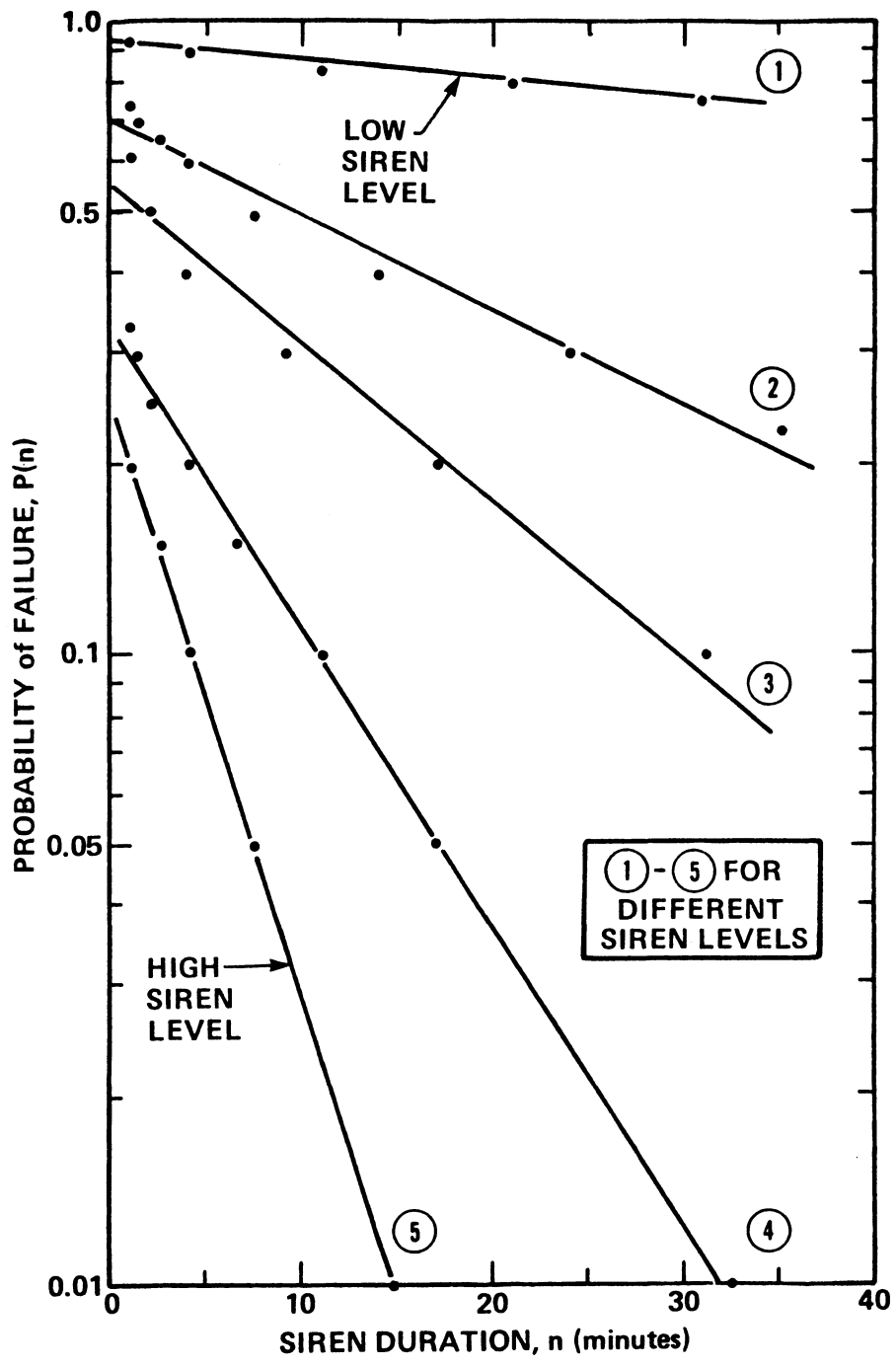
FIG. E-7. LOGARITHM OF THE PROBABILITY OF SIREN FAILURE-TO-ALERT VS. SIREN DURATION FOR FIVE DIFFERENT SIREN LEVELS, DERIVED FROM THE DATA IN TABLE E.1.
